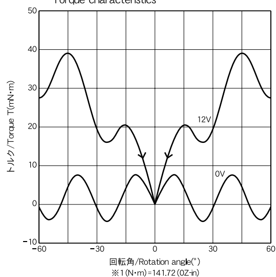
Torque characteristics
